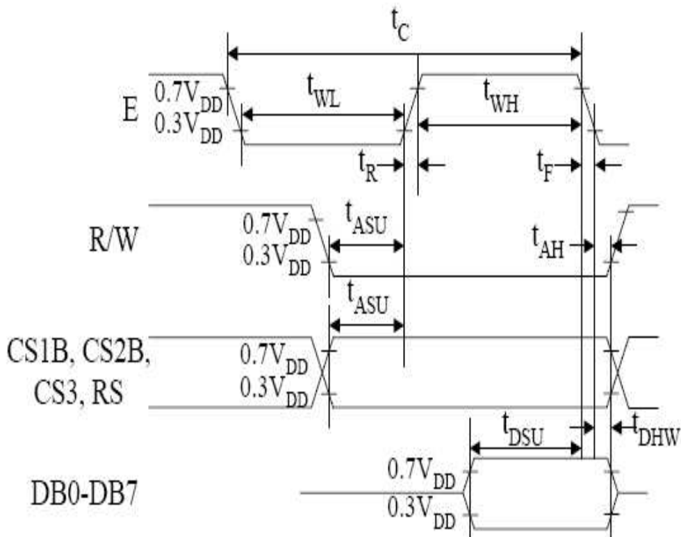
MPU Write Timing
